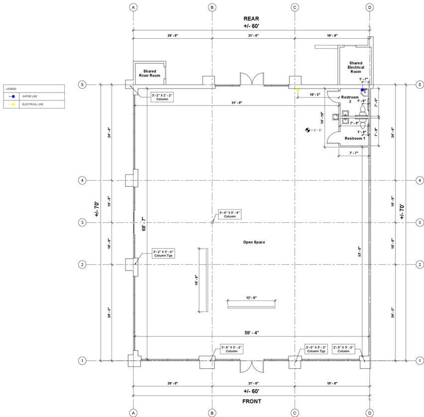
A1 MAIN FLOOR
